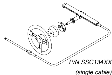
"The Rack" Back Mount Single Station System (Steering Wheel not included.)
