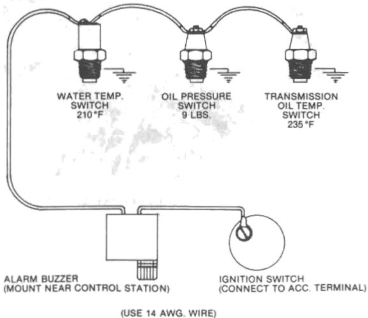
Figure 27. Standard Engine Alarm System
