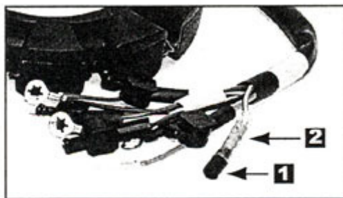
1 - Bullet Connector (RED/WHITE LEAD) 2 - Sealing Plug
