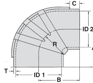
90° Reducing Elbow
